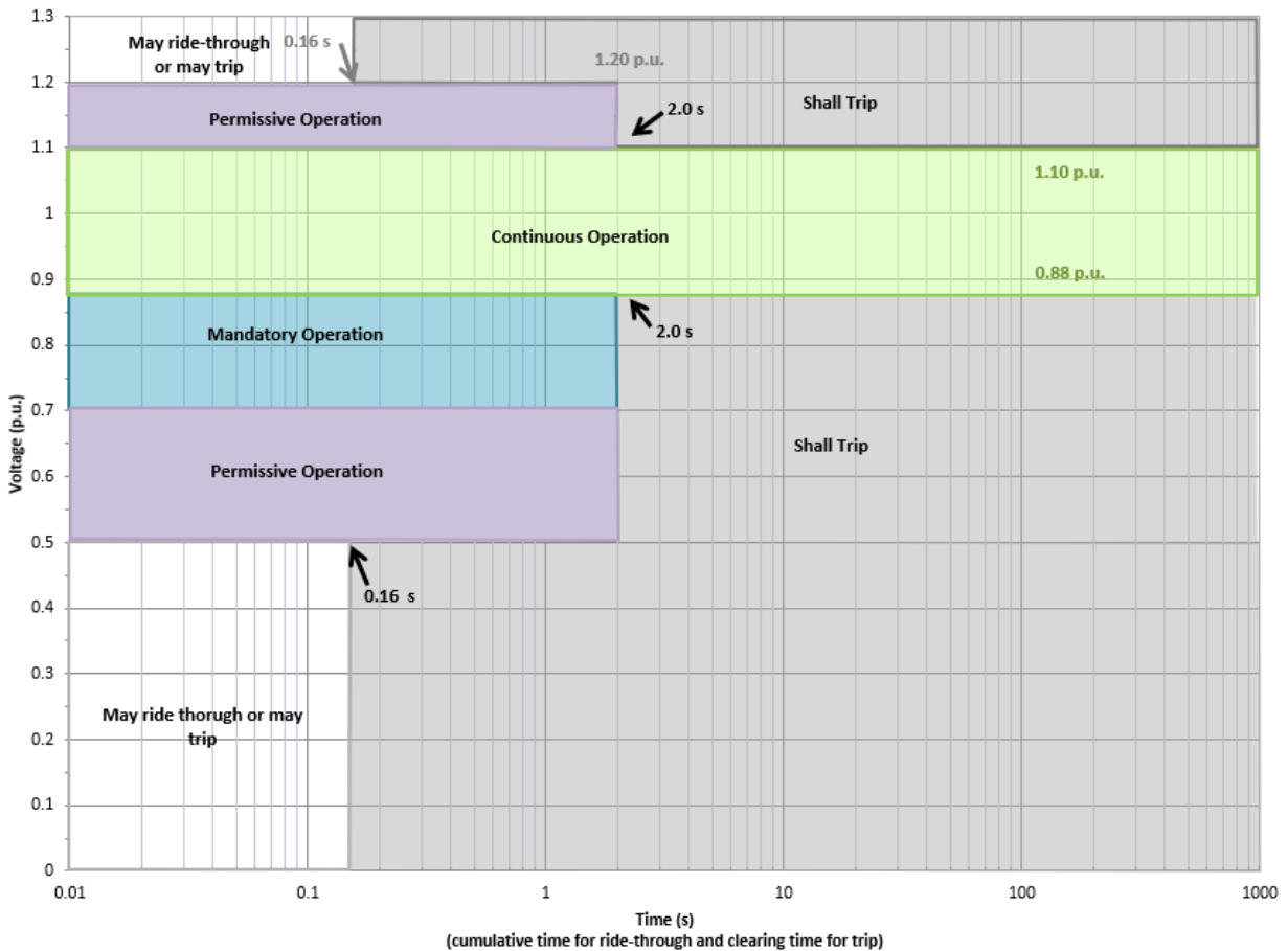
Figure 3: Voltage ride-through and trip requirements for non- inverter based DER abnormal operating performance - Category I 4
